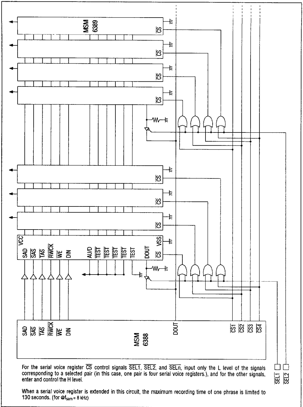
Circuit Diagram 5
