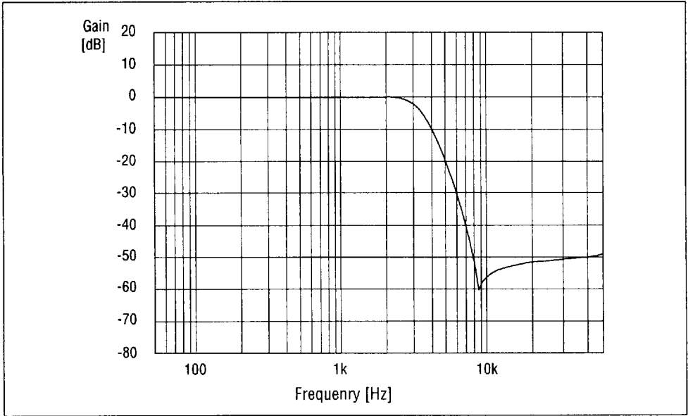
LPF Frequency Characteristics ( f_{sam}=8.0kHz )
